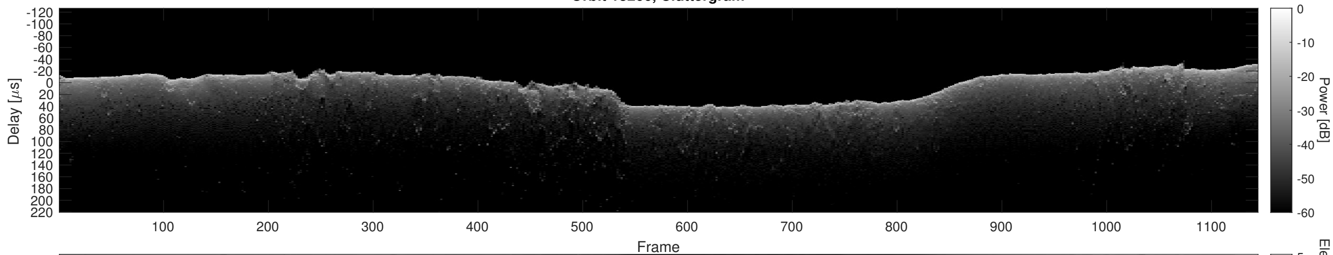
Orbit 13266, Cluttergram
