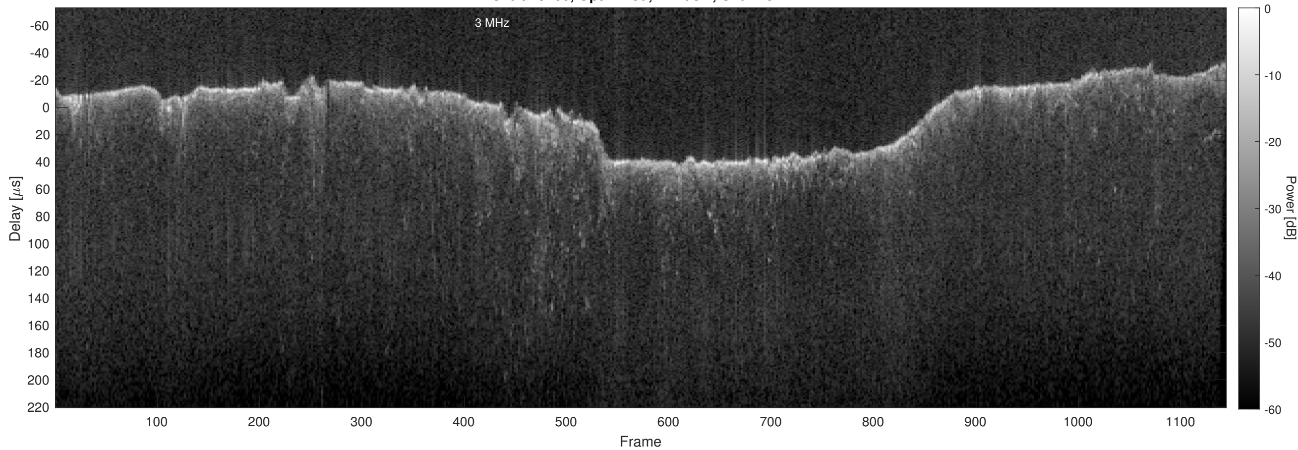
Orbit 13266, Optimized, Window, Channel 2
