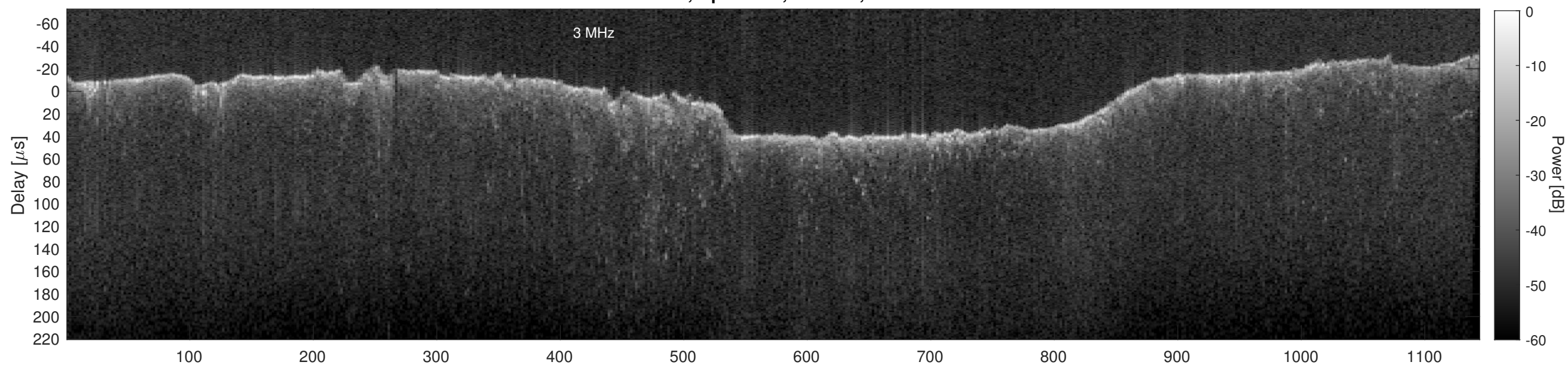
Orbit 13266, Cluttergram
