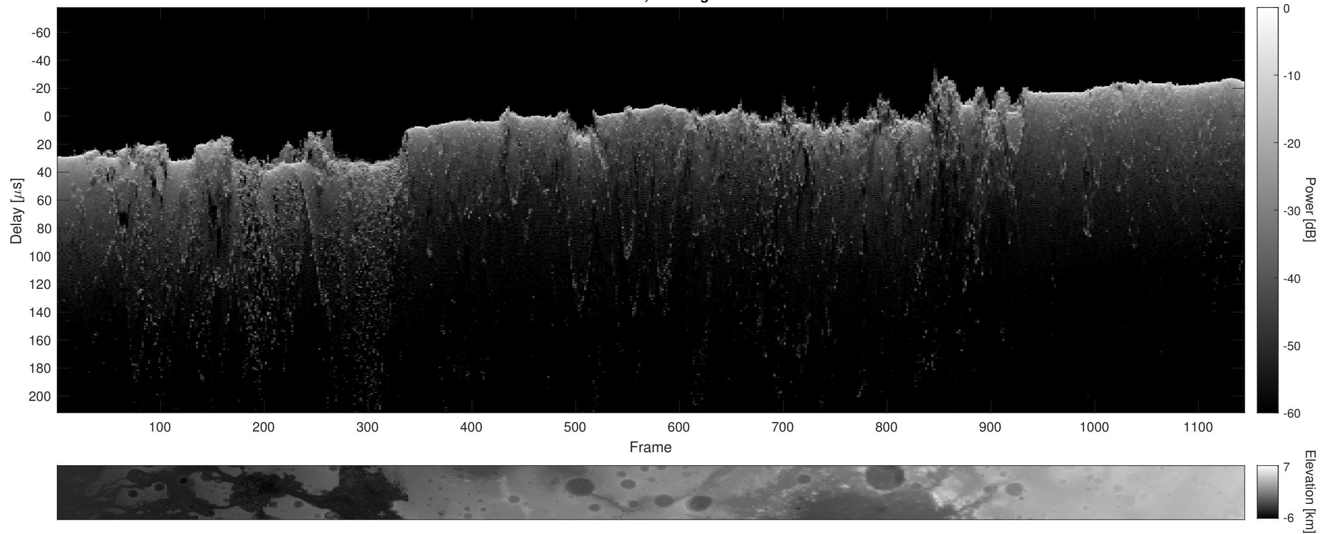
Orbit 13267, Cluttergram
