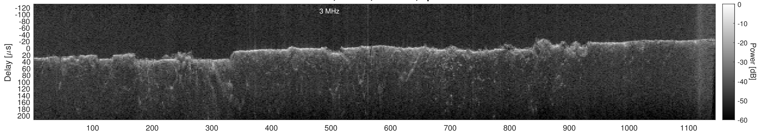
Orbit 13267, Cluttergram
