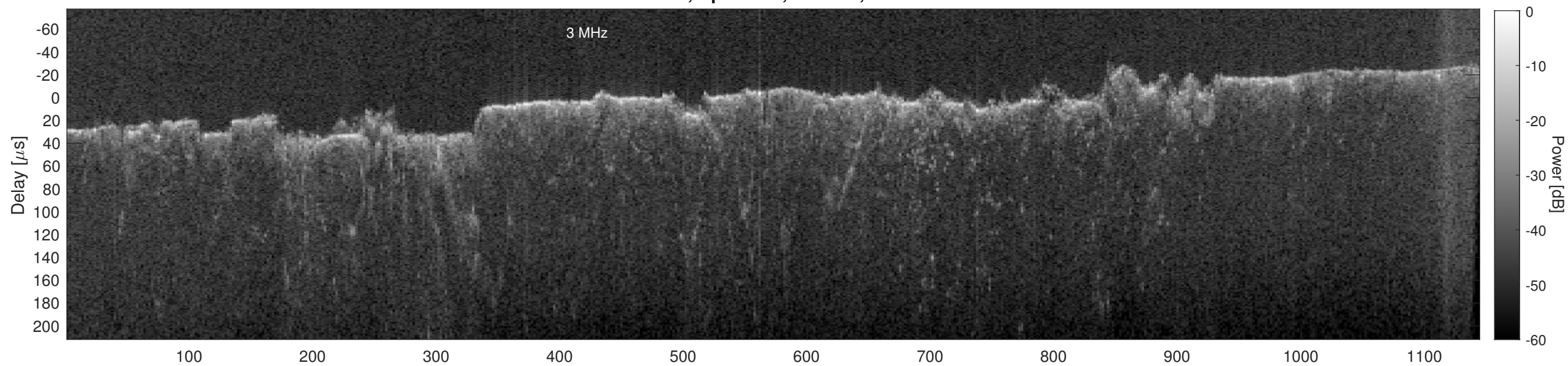
Orbit 13267, Cluttergram
