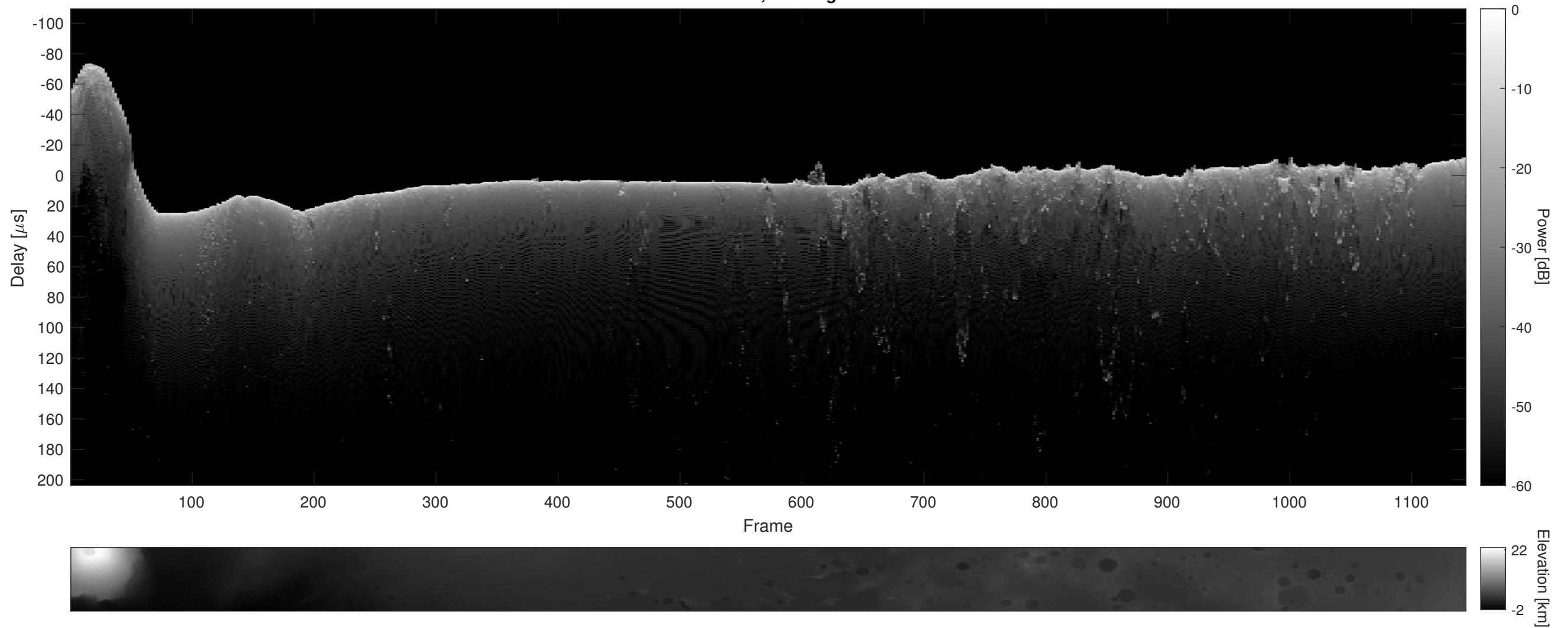
Orbit 13268, Cluttergram
