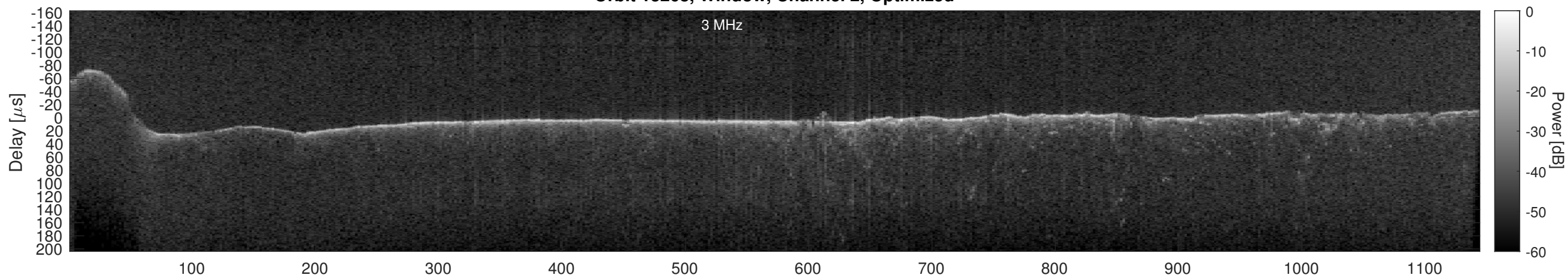
Orbit 13268, Cluttergram
