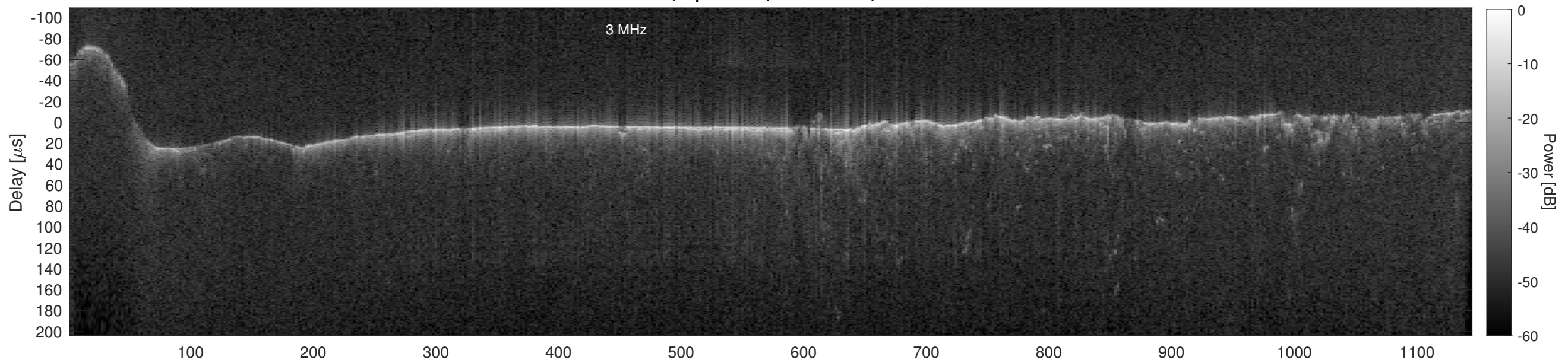
Orbit 13268, Cluttergram
