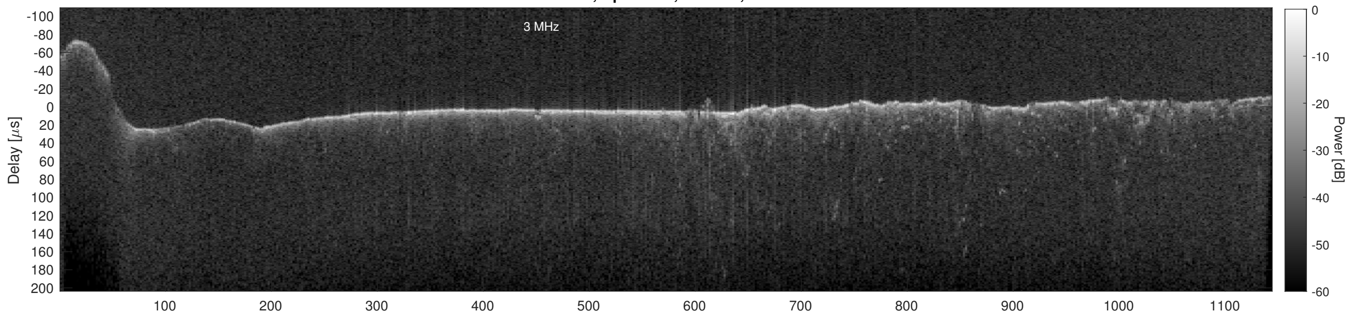
Orbit 13268, Cluttergram
