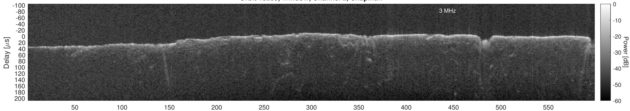
Orbit 13269, Window, Channel 2, Optimized
