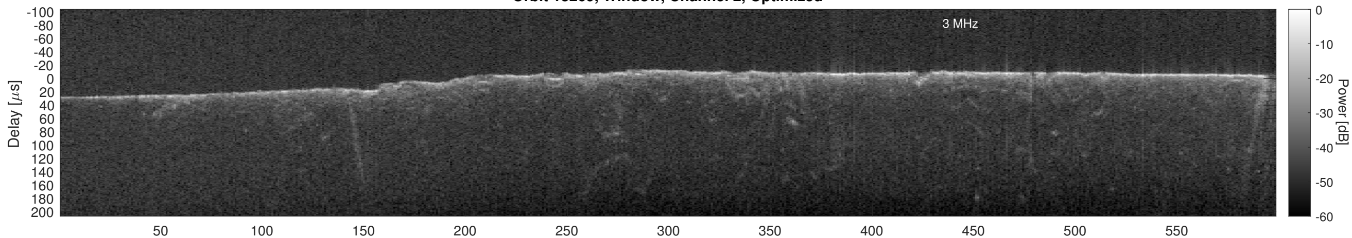
Orbit 13269, Cluttergram
