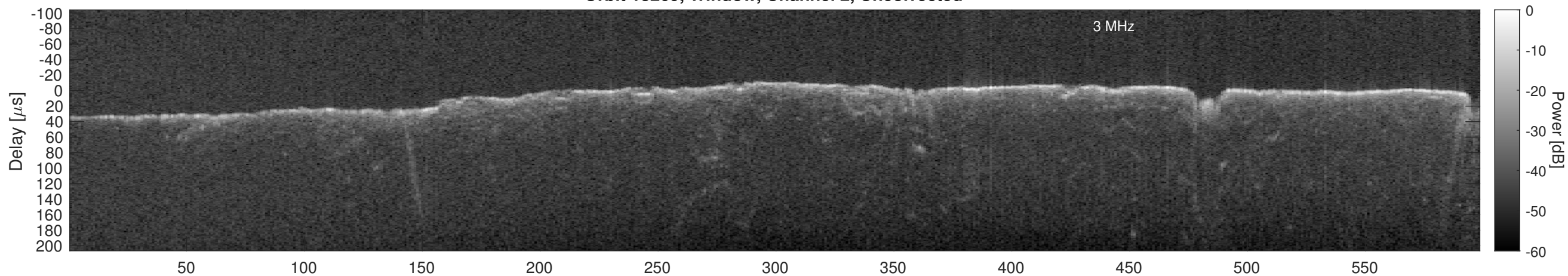
Orbit 13269, Window, Channel 2, Chapman
