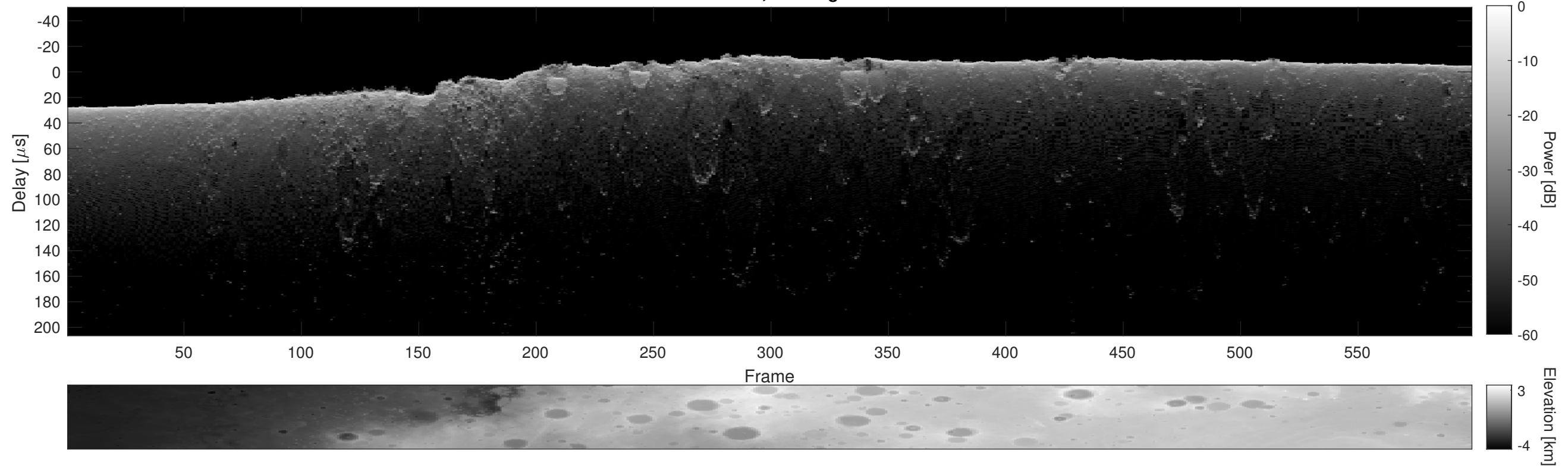
Orbit 13269, Cluttergram
