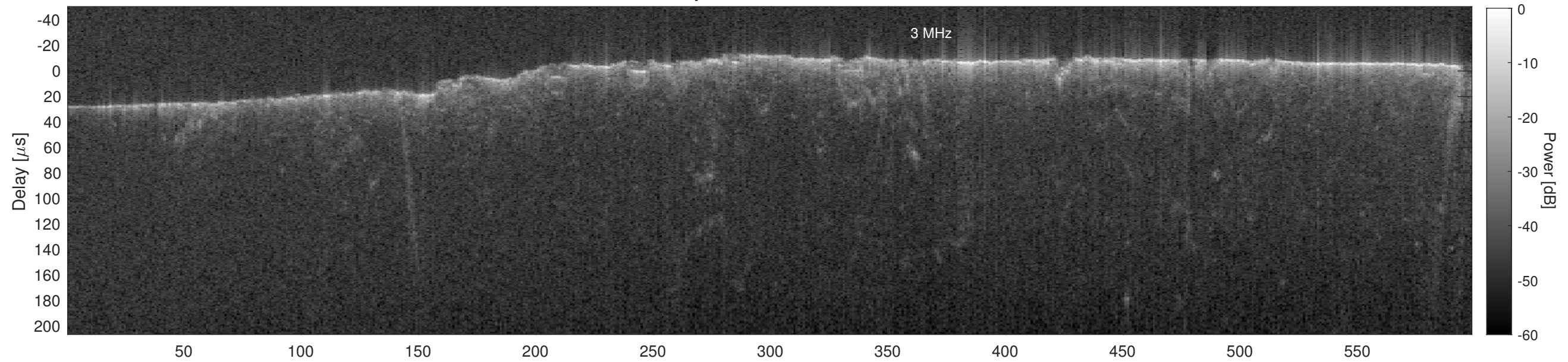
Orbit 13269, Cluttergram
