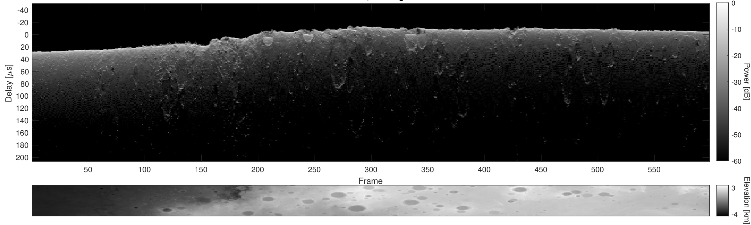
Orbit 13269, Cluttergram
