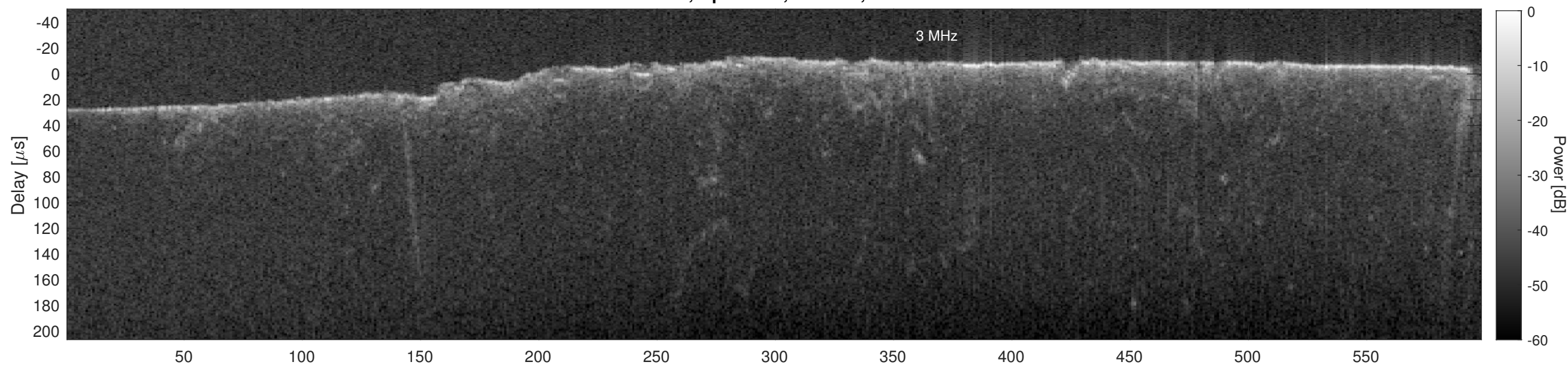
Orbit 13269, Cluttergram
