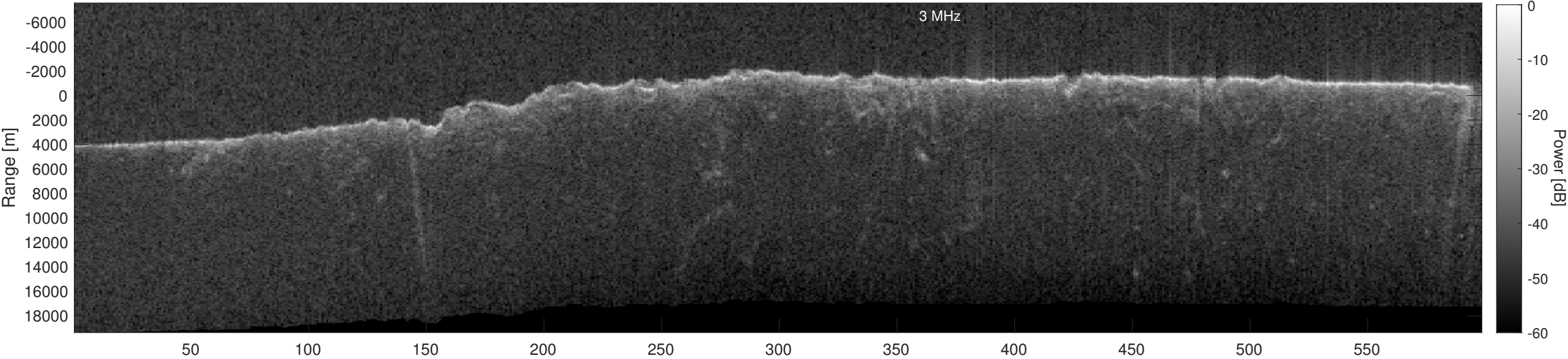
Orbit 13269, Depth-Corrected Cluttergram
