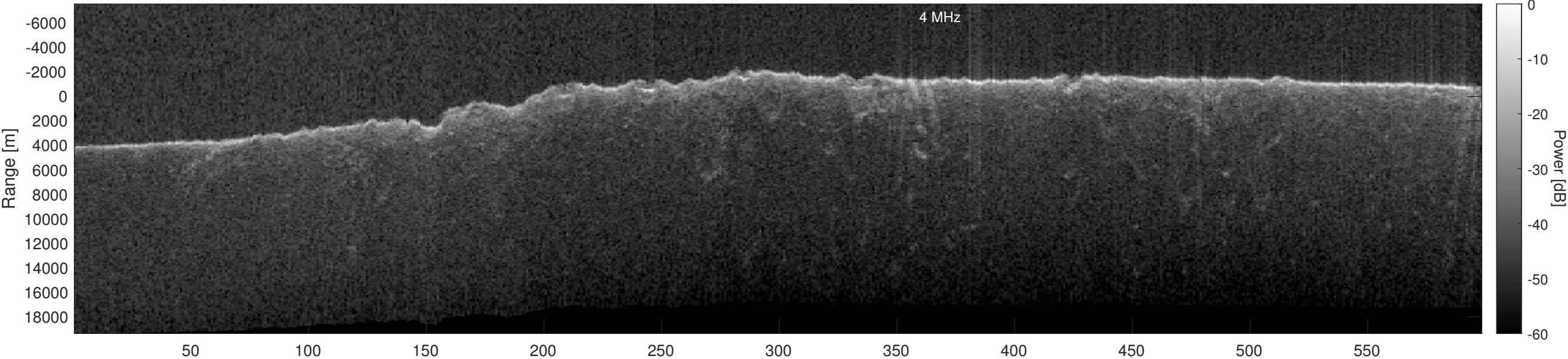
Orbit 13269, Optimized, Window, Depth-Corrected, Channel 2
