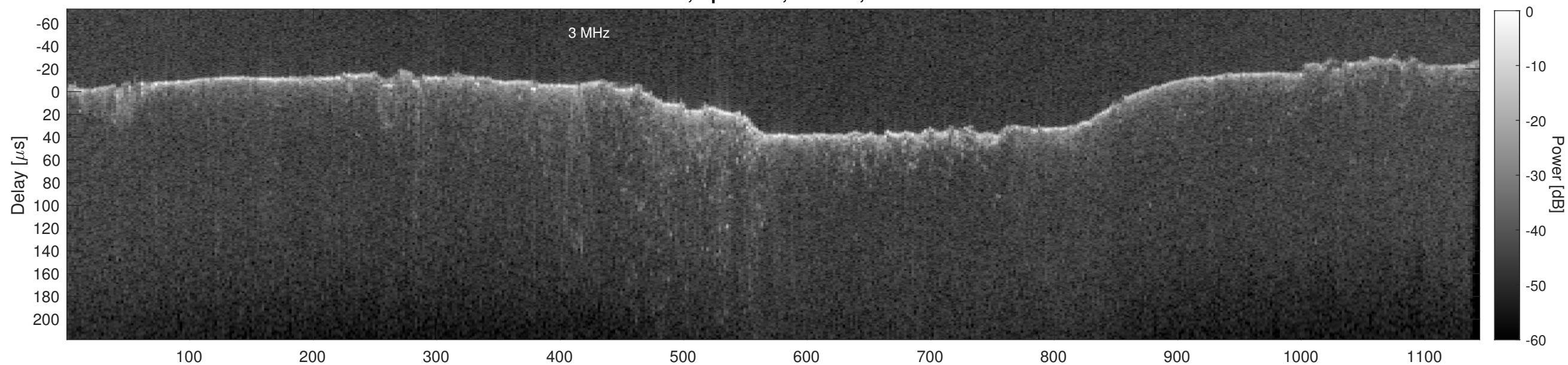
Orbit 13273, Cluttergram
