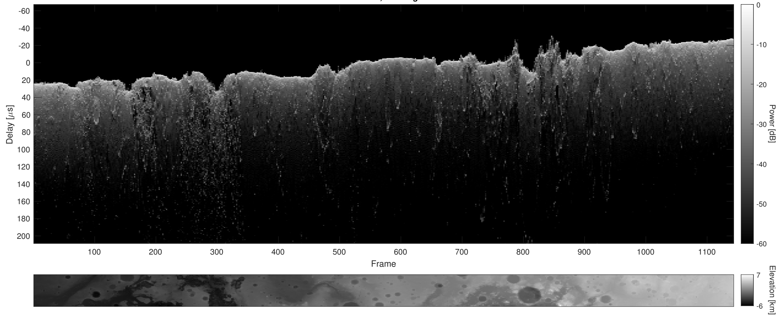
Orbit 13274, Cluttergram
