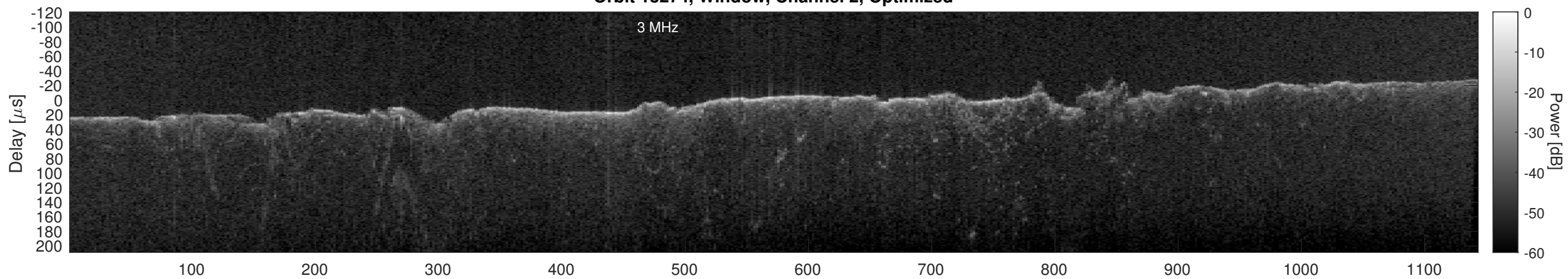
Orbit 13274, Cluttergram
