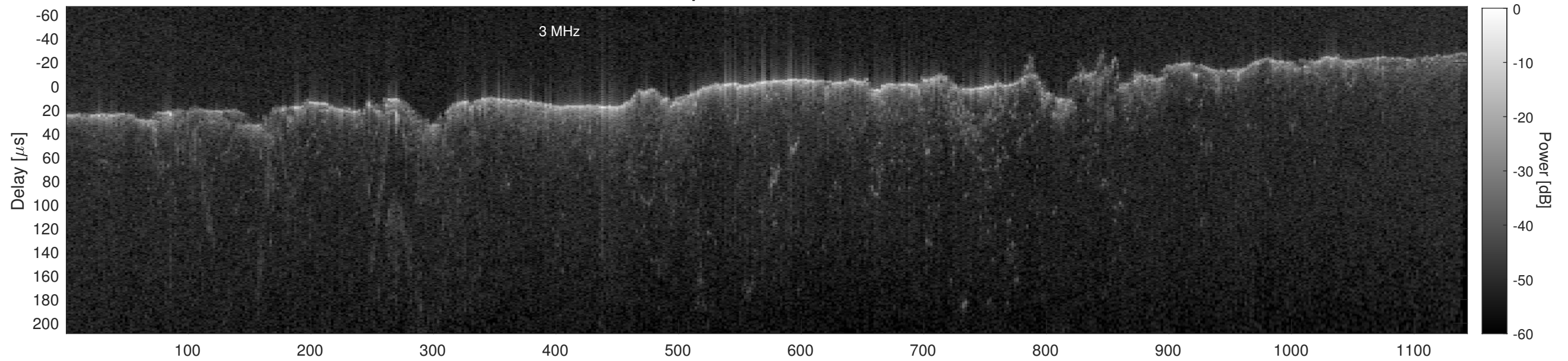
Orbit 13274, Cluttergram
