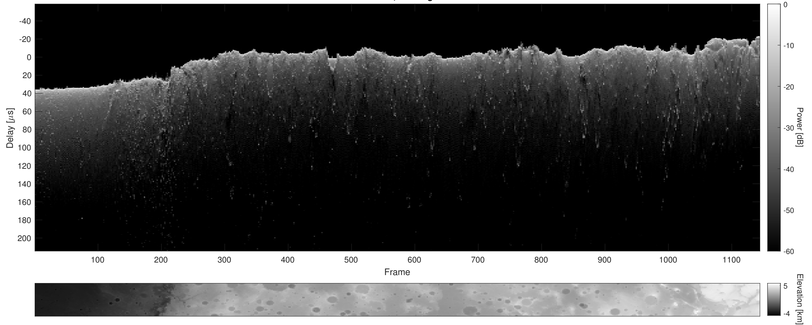
Orbit 13276, Cluttergram
