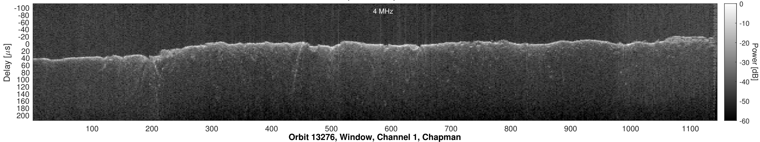
Orbit 13276, Channel 1, Uncorrected
