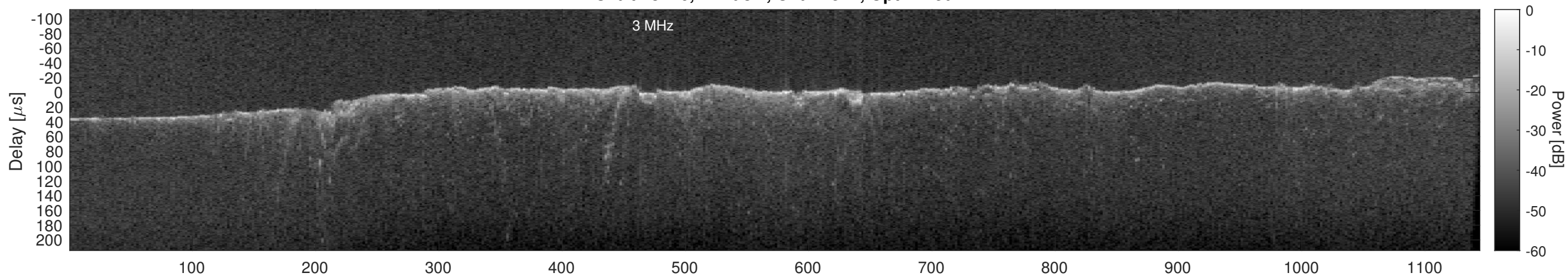
Orbit 13276, Cluttergram
