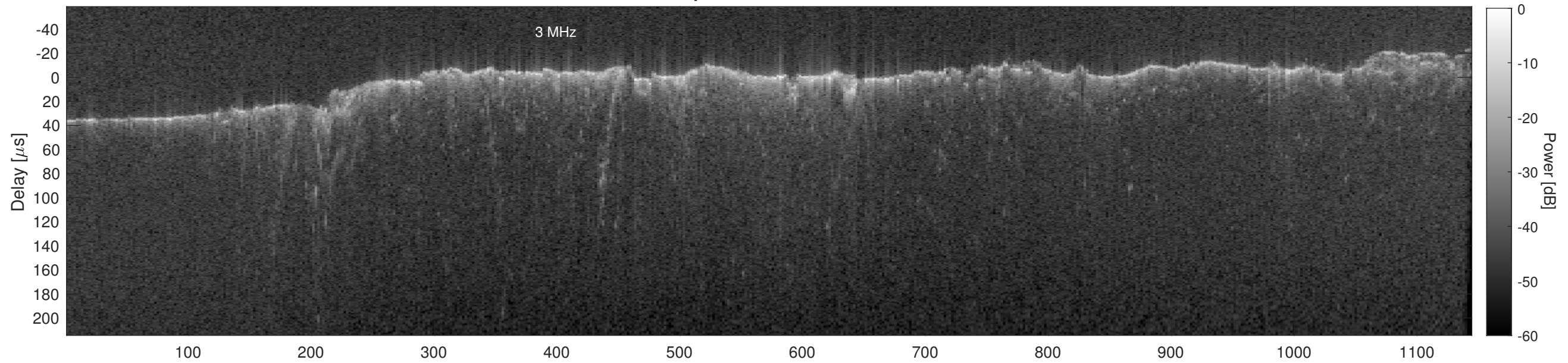
Orbit 13276, Cluttergram
