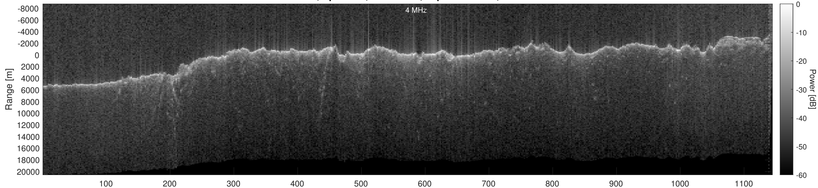
Orbit 13276, Optimized, No Window, Depth-Corrected, Channel 2
