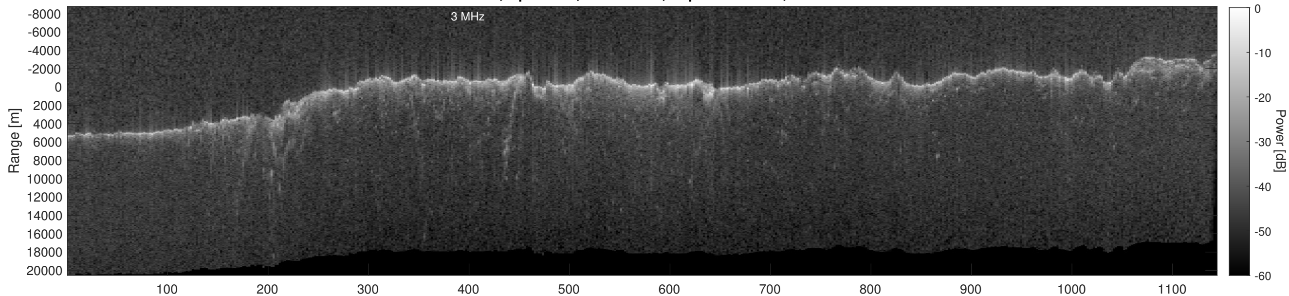
Orbit 13276, Depth-Corrected Cluttergram
