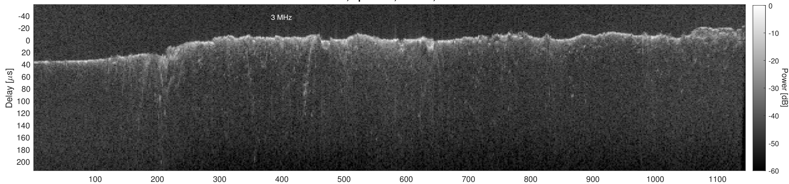
Orbit 13276, Cluttergram
