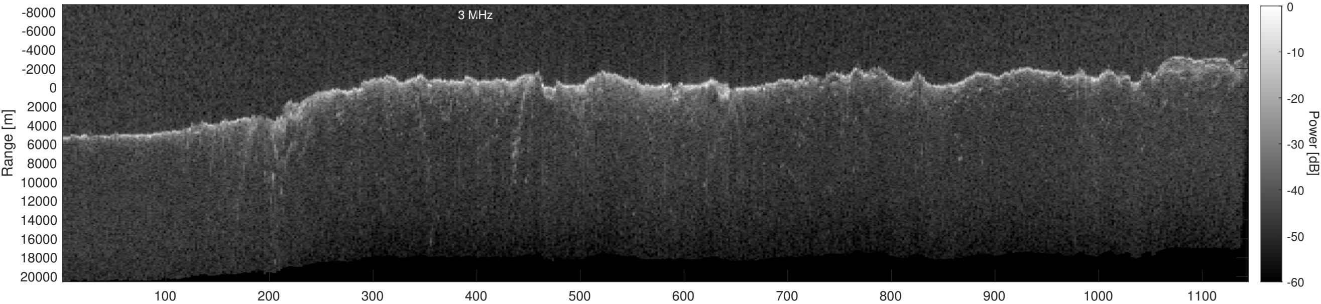
Orbit 13276, Depth-Corrected Cluttergram
