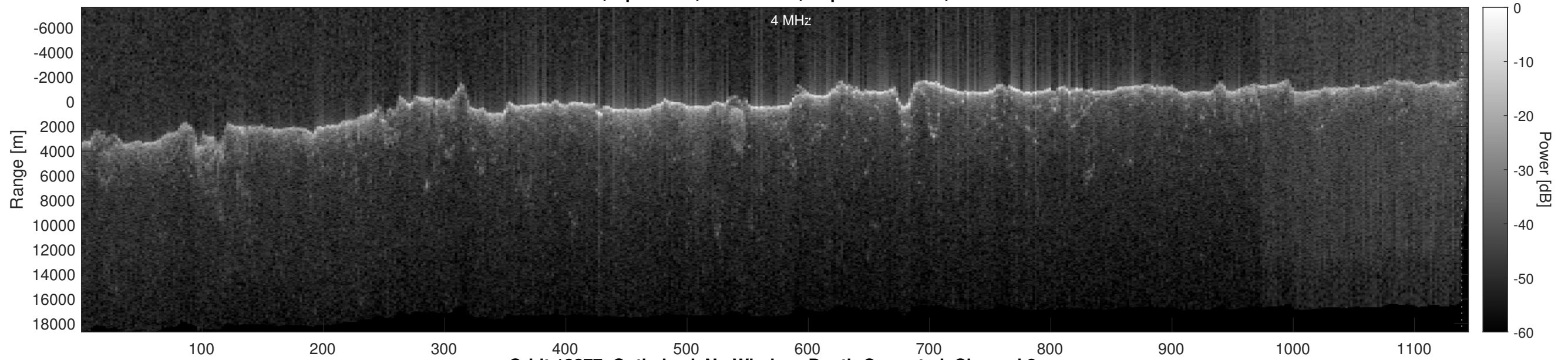
Orbit 13277, Optimized, No Window, Depth-Corrected, Channel 2
