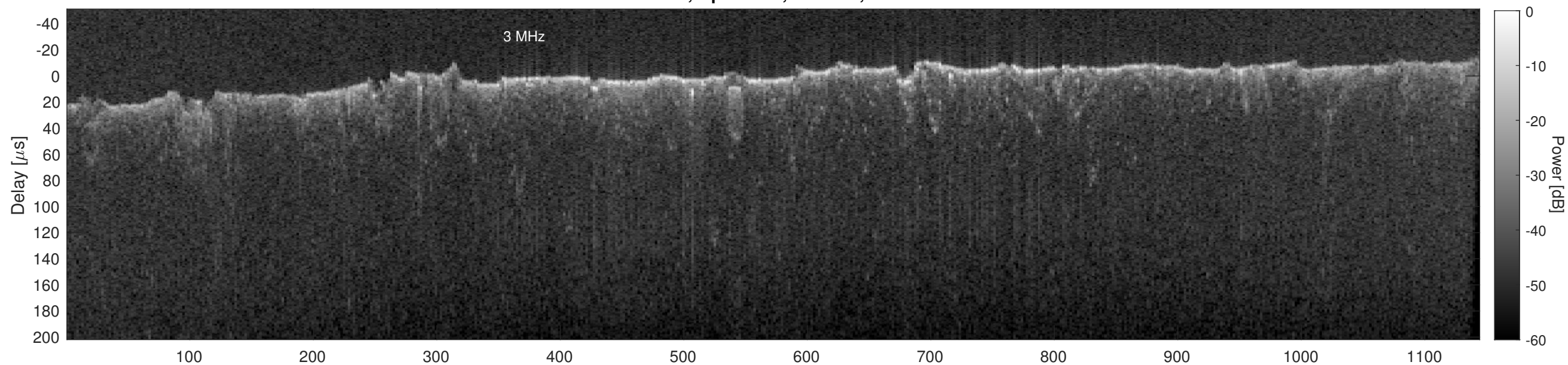
Orbit 13277, Cluttergram
