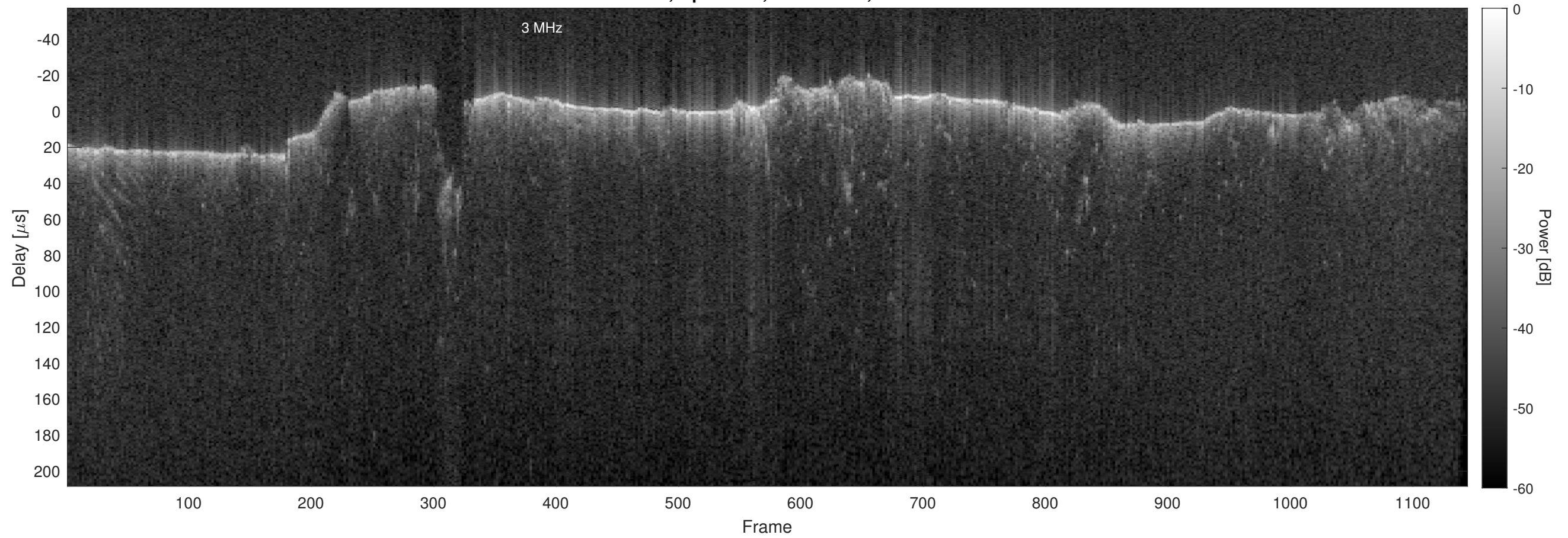
Orbit 13278, Optimized, No Window, Channel 2
