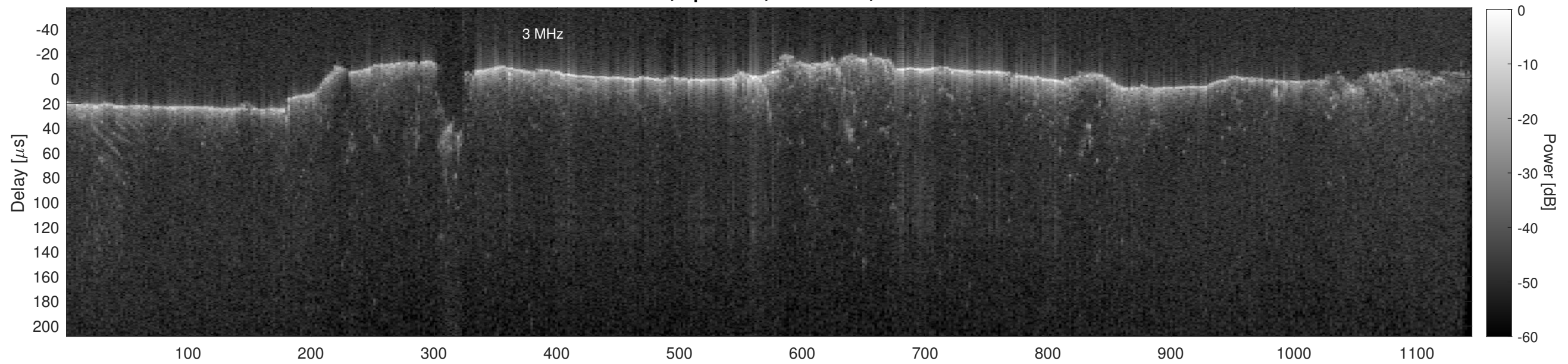
Orbit 13278, Cluttergram
