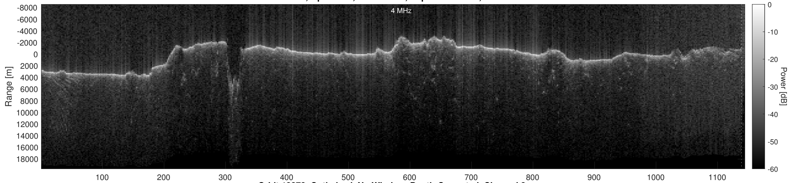
Orbit 13278, Optimized, No Window, Depth-Corrected, Channel 2
