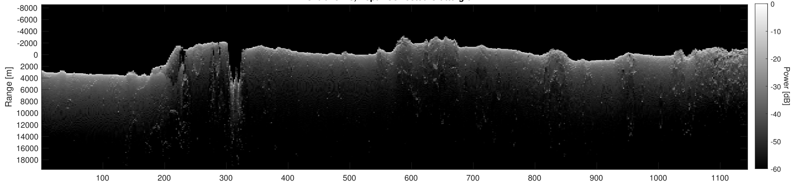
Orbit 13278, Depth-Corrected Cluttergram
