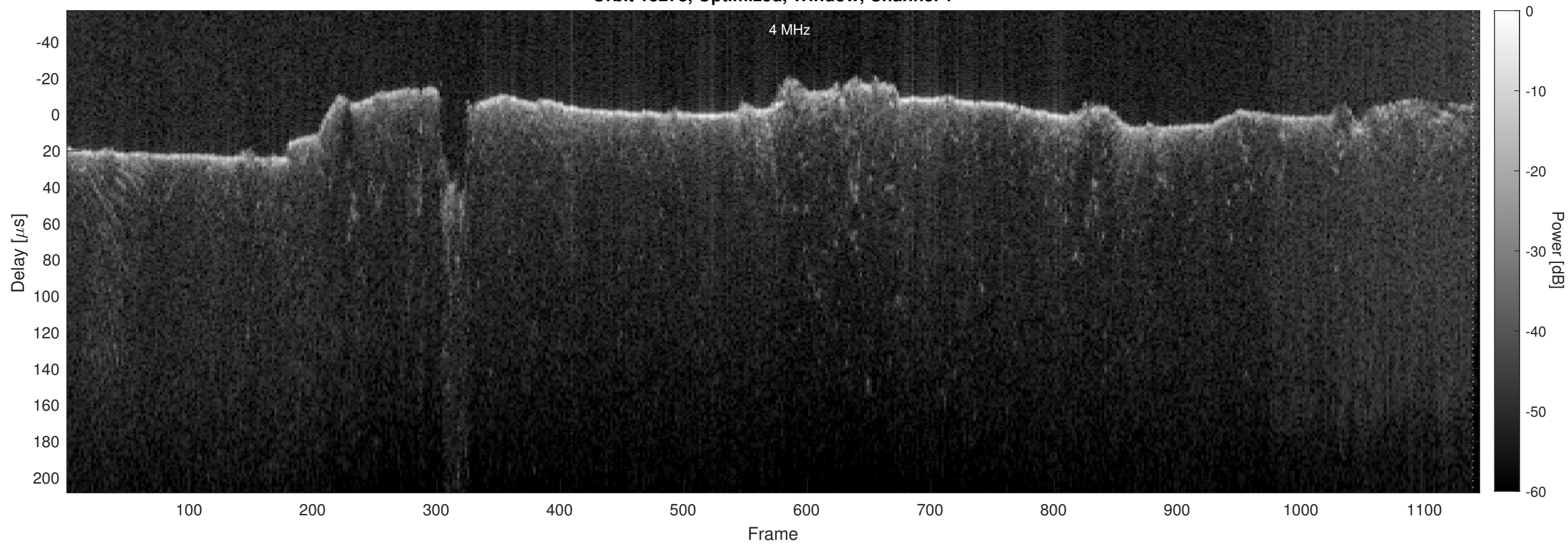
Orbit 13278, Optimized, Window, Channel 2
