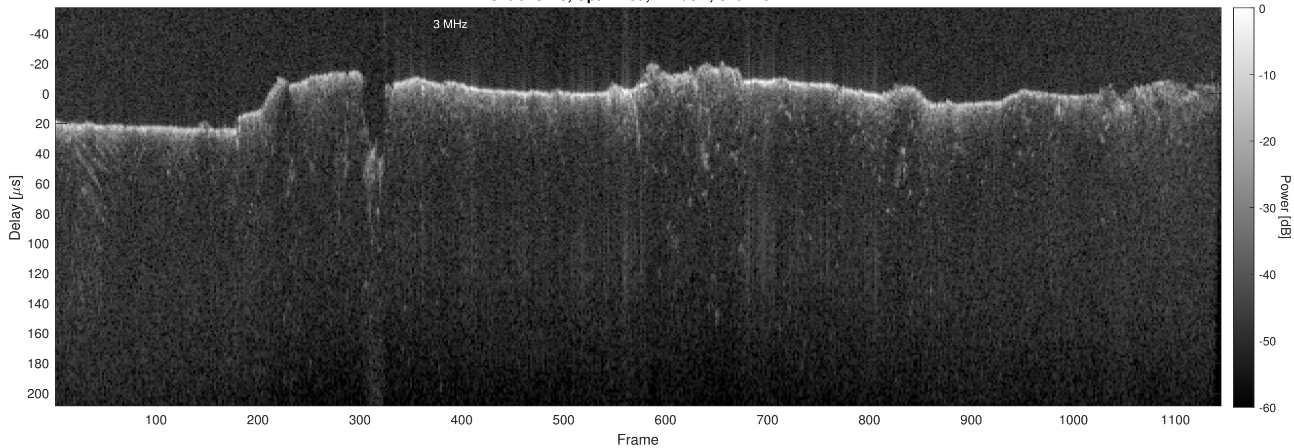
Orbit 13278, Optimized, Window, Channel 2
