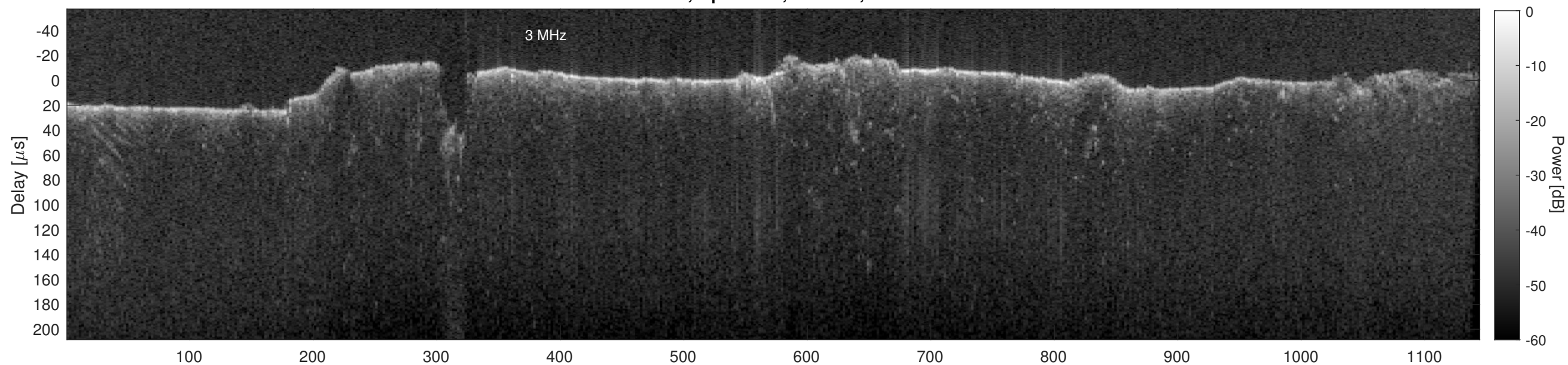
Orbit 13278, Cluttergram
