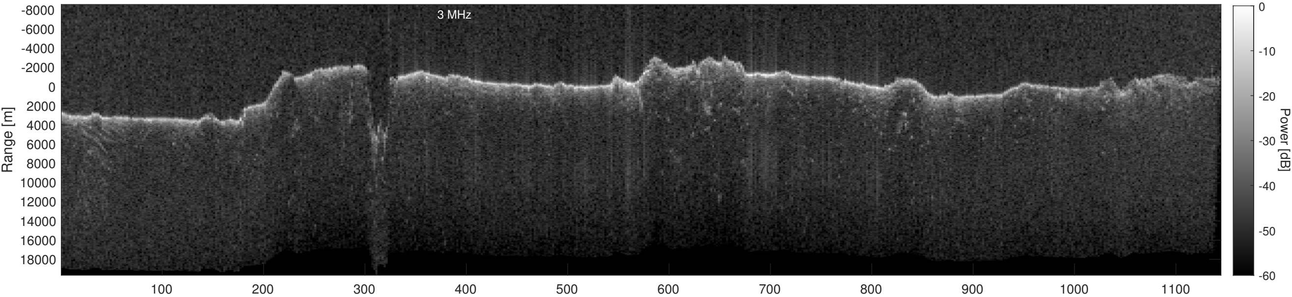
Orbit 13278, Depth-Corrected Cluttergram
