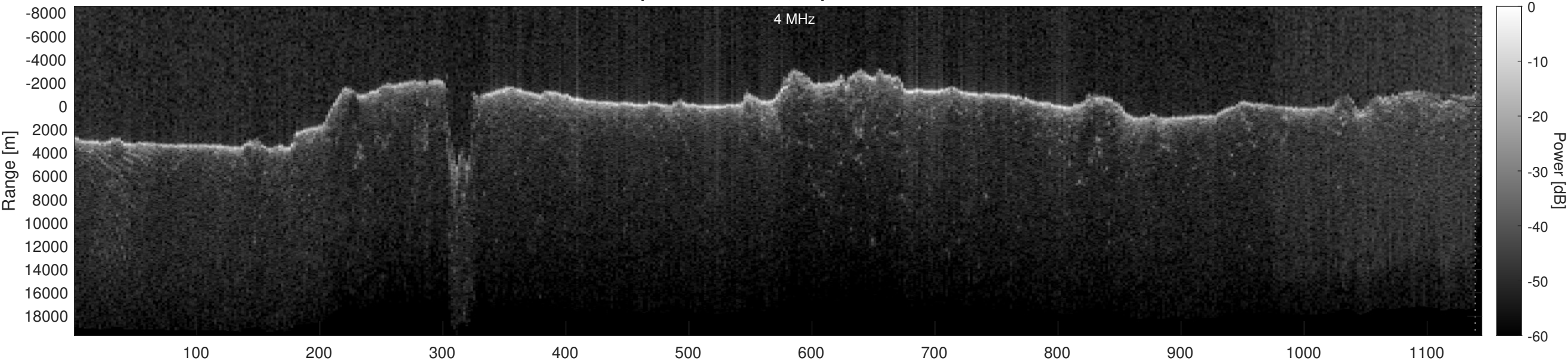
Orbit 13278, Optimized, Window, Depth-Corrected, Channel 2
