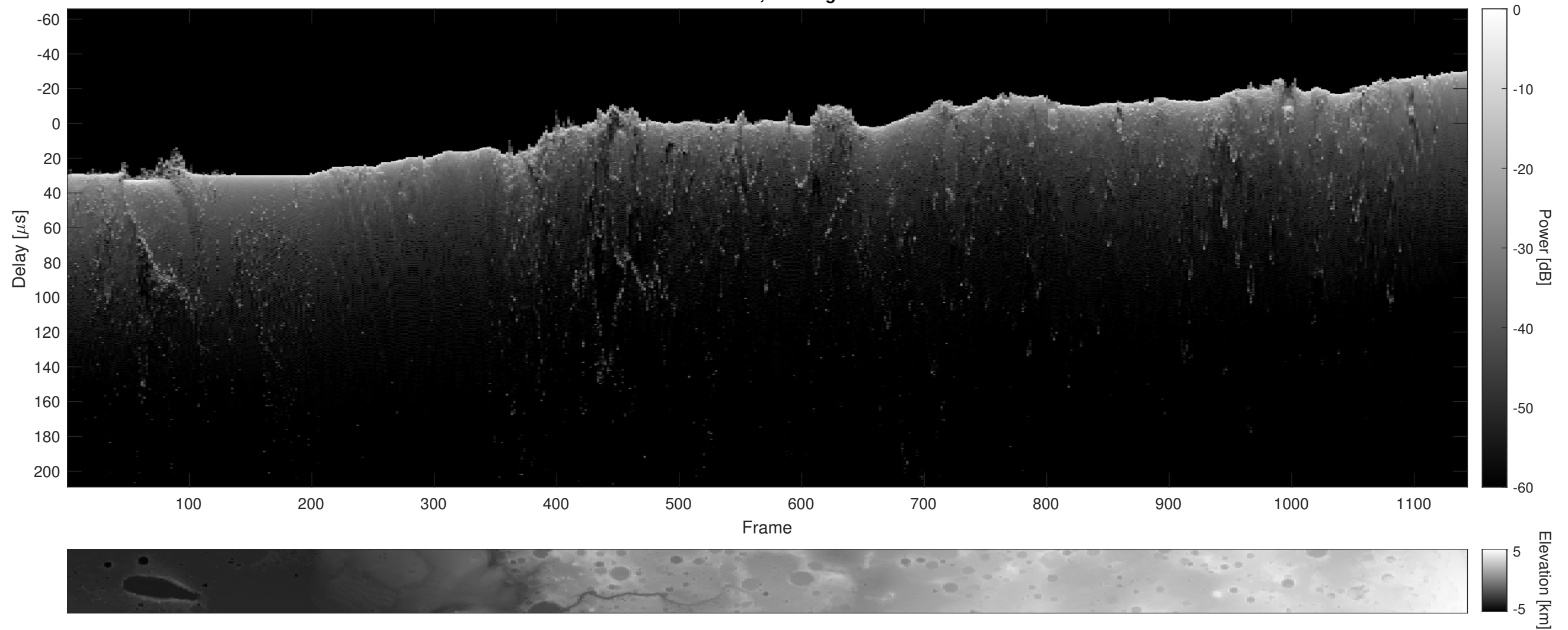
Orbit 13279, Cluttergram
