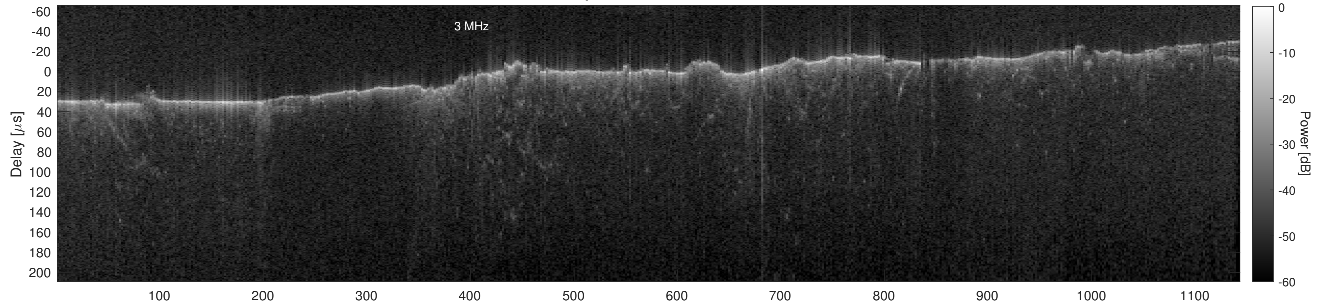
Orbit 13279, Cluttergram
