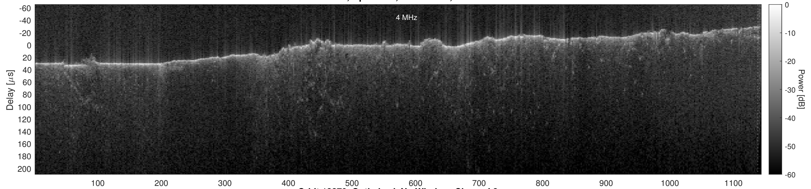
Orbit 13279, Optimized, No Window, Channel 2
