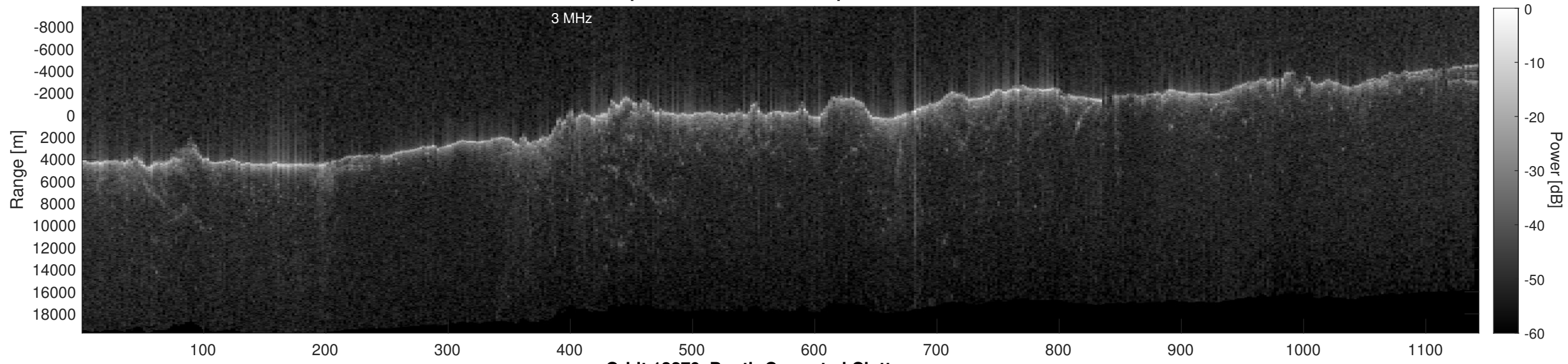
Orbit 13279, Depth-Corrected Cluttergram
