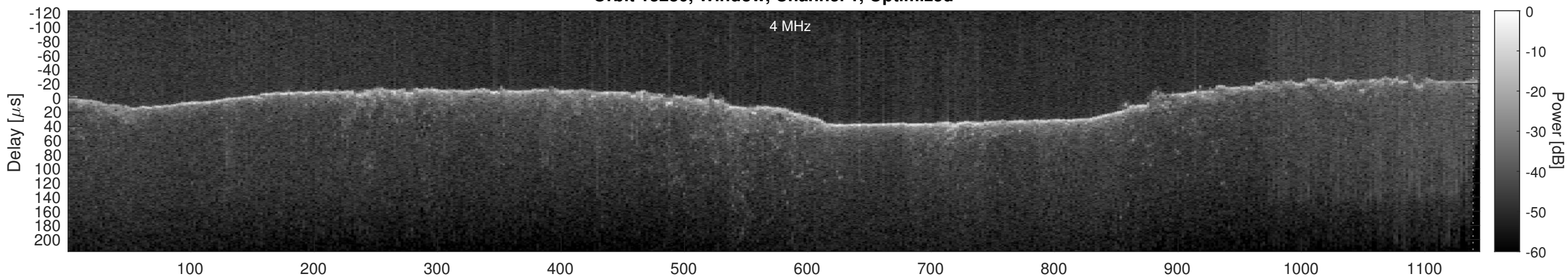
Orbit 13280, Cluttergram
