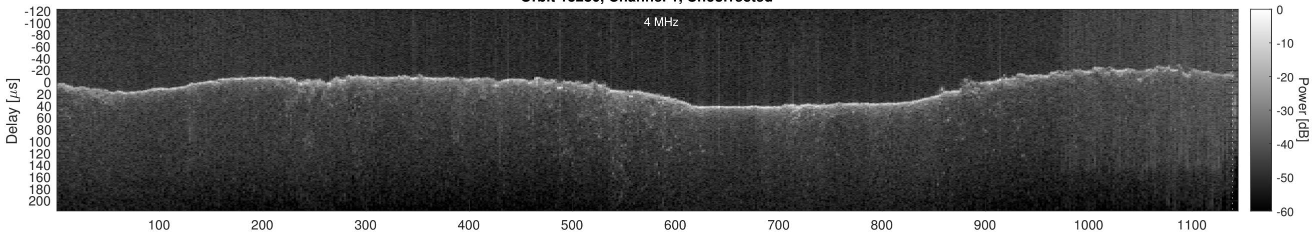
Orbit 13280, Window, Channel 1, Chapman
