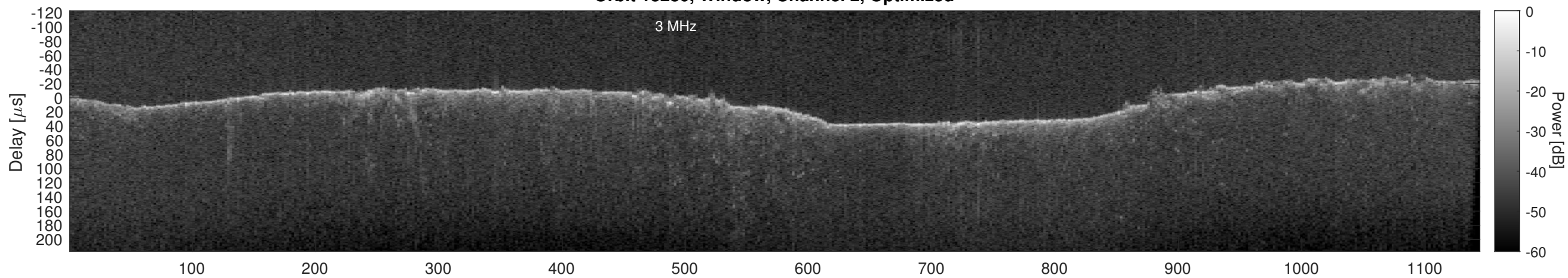
Orbit 13280, Cluttergram
