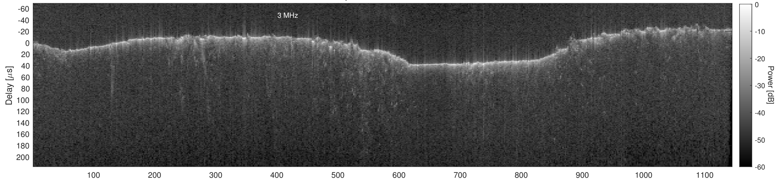
Orbit 13280, Cluttergram
