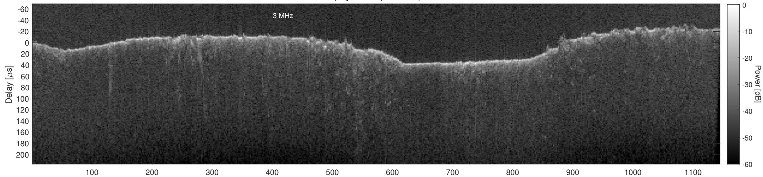
Orbit 13280, Cluttergram
