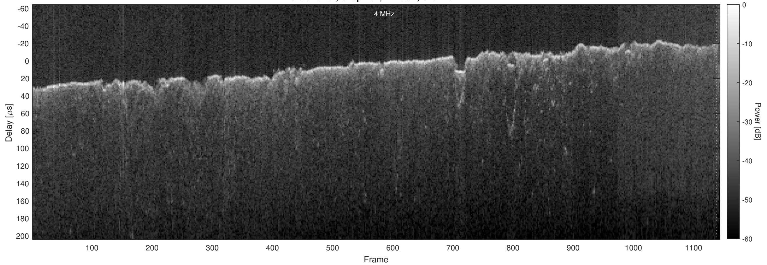
Orbit 13281, Chapman, Window, Channel 2
