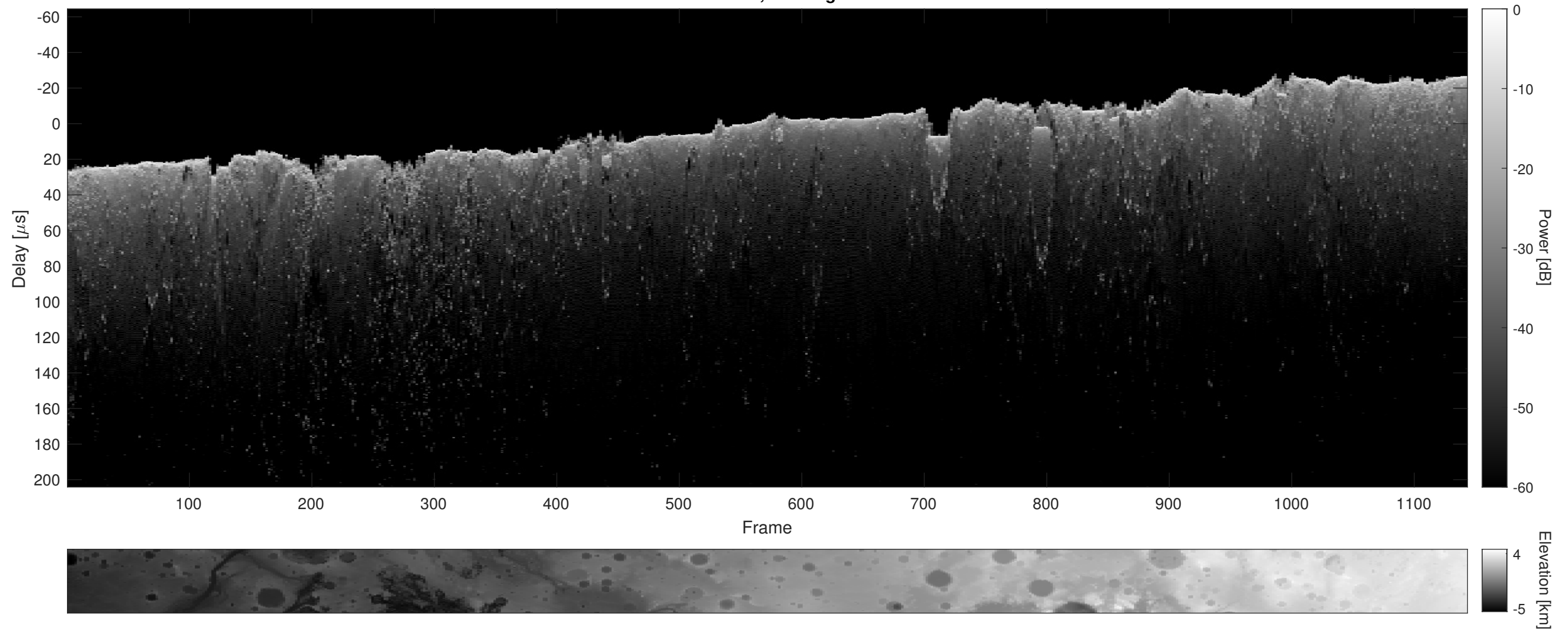
Orbit 13281, Cluttergram
