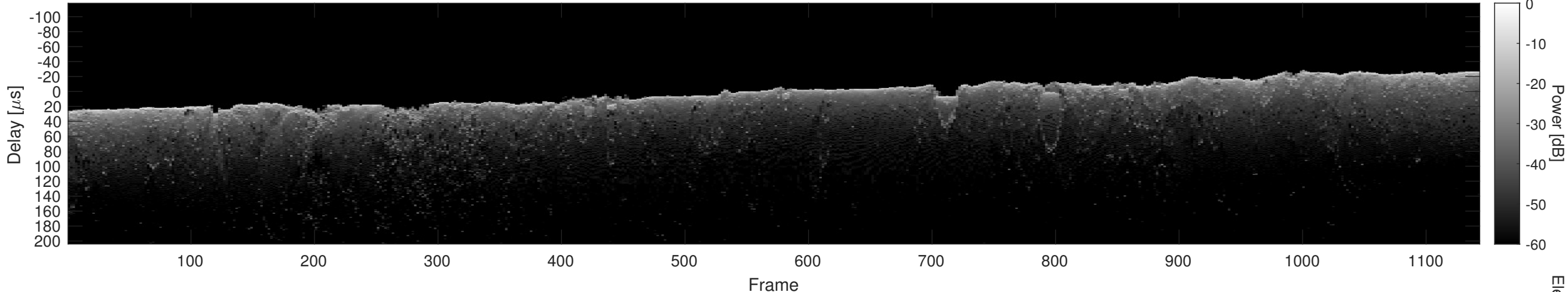
Orbit 13281, Cluttergram
