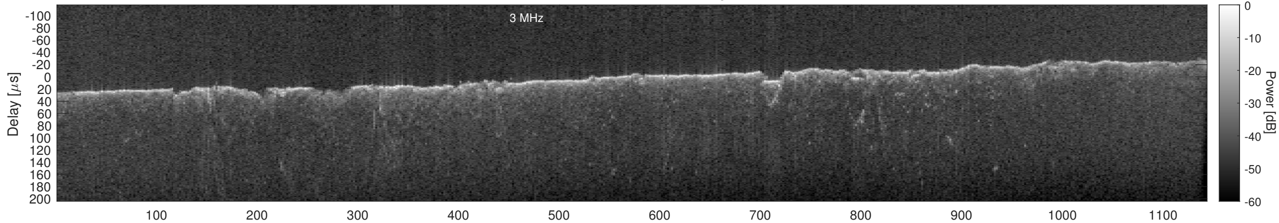
Orbit 13281, Cluttergram
