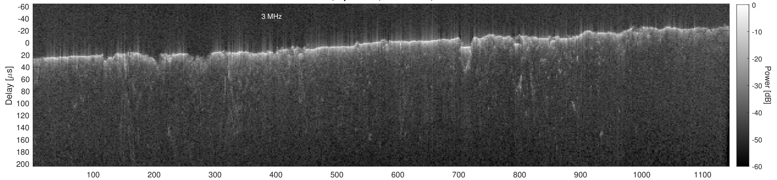
Orbit 13281, Cluttergram
