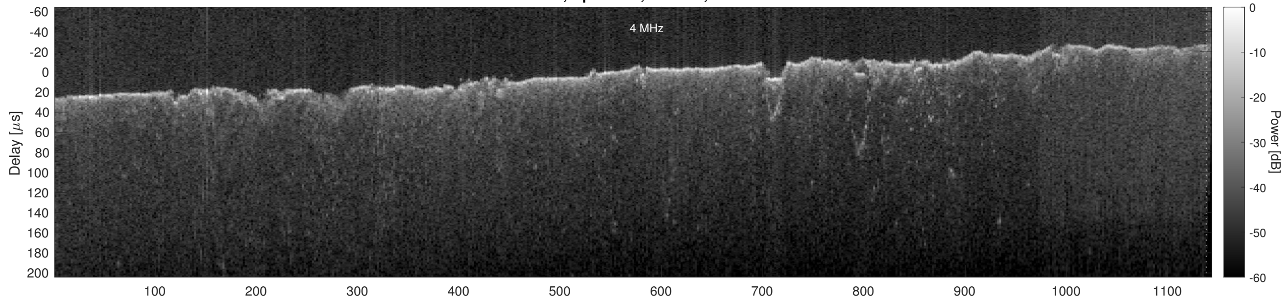
Orbit 13281, Optimized, Window, Channel 2
