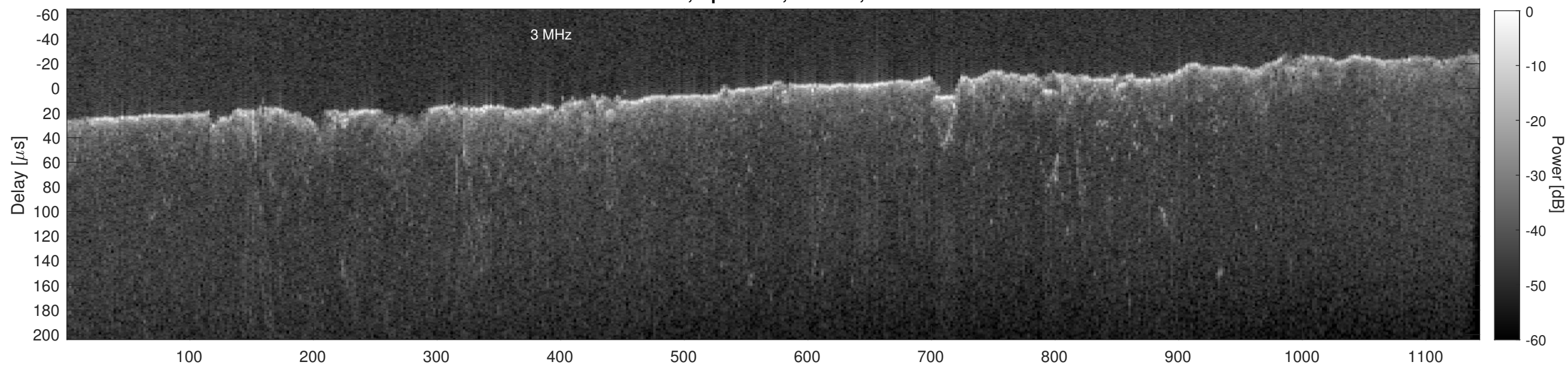
Orbit 13281, Cluttergram
