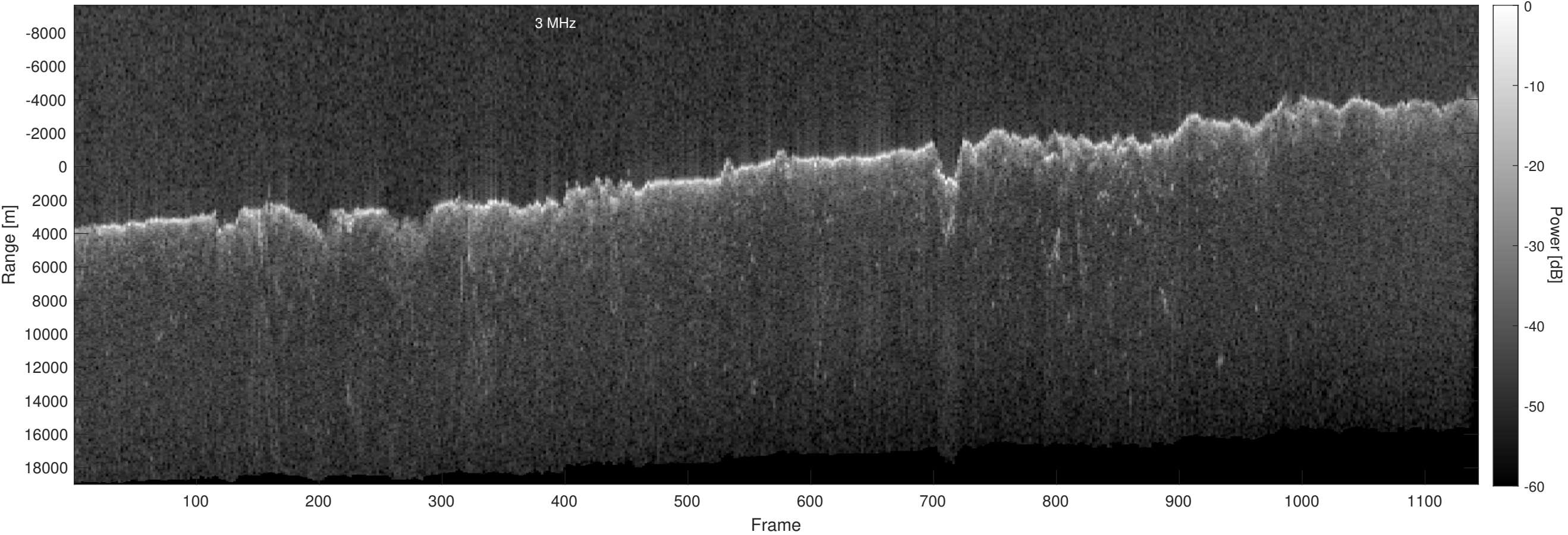
Orbit 13281, Optimized, Window, Depth-Corrected, Channel 2
