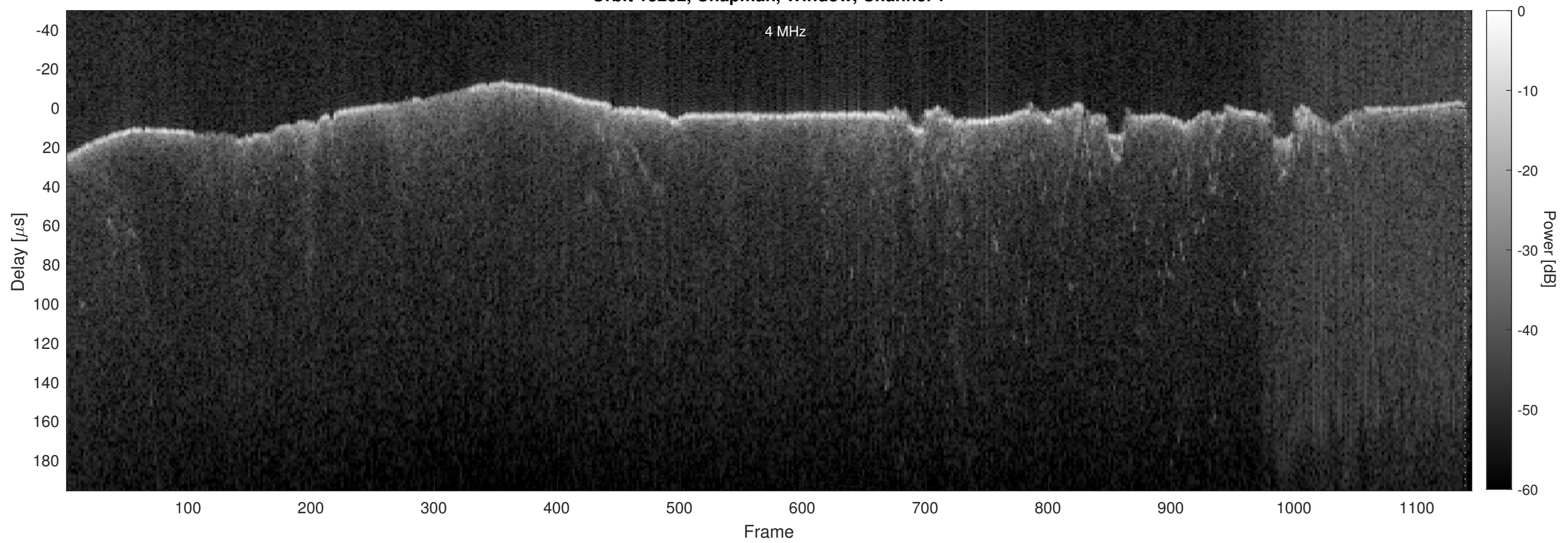
Orbit 13282, Chapman, Window, Channel 2
