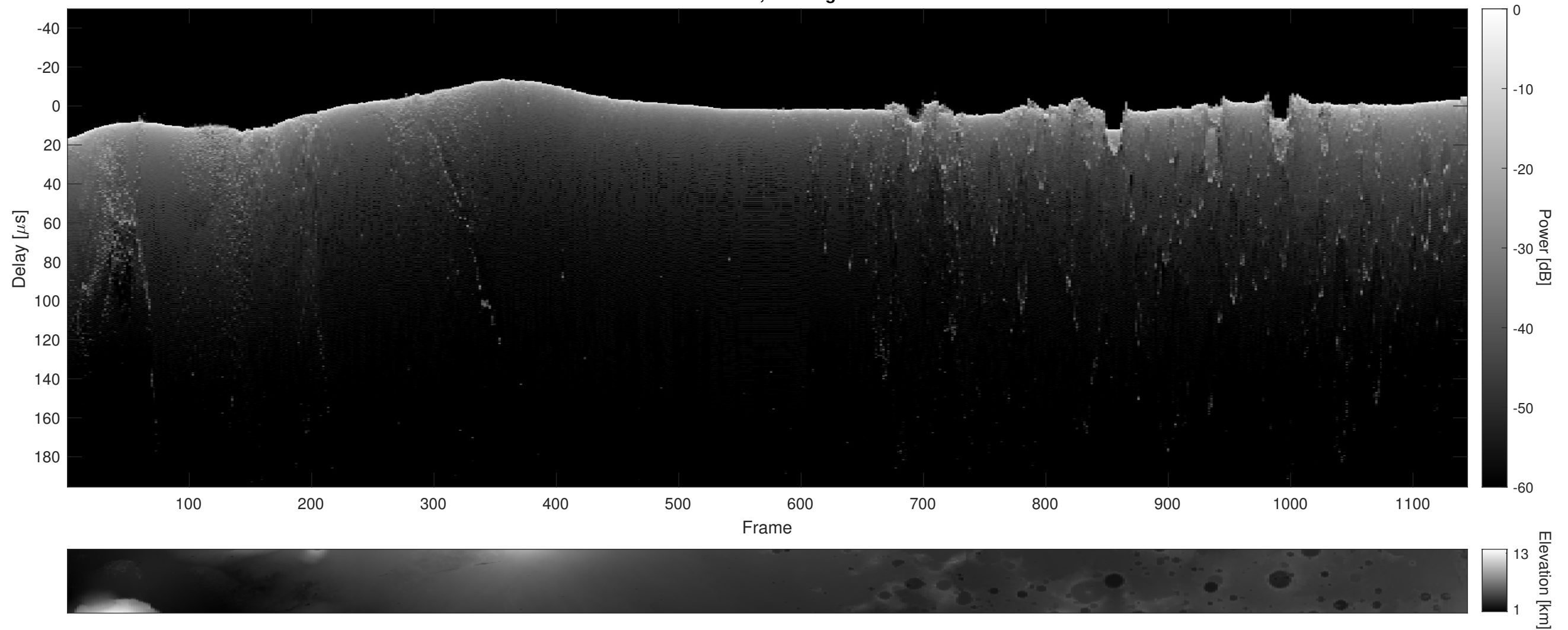
Orbit 13282, Cluttergram
