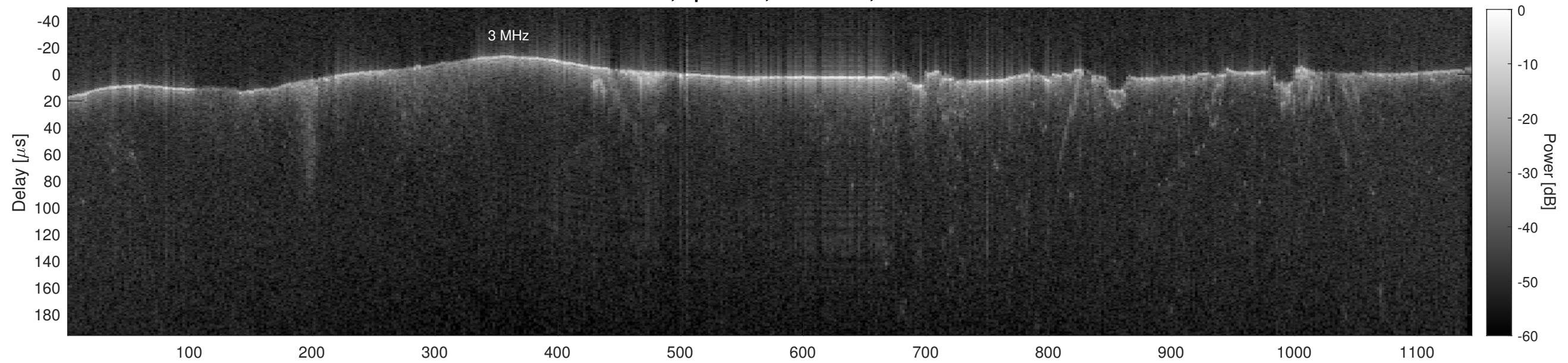
Orbit 13282, Cluttergram
